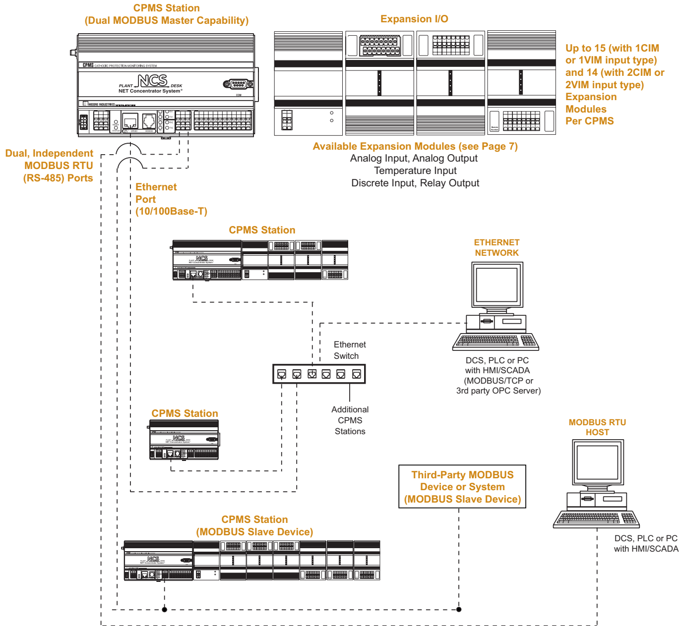
Figure 4. Expansion I/O (see Page 7) allows each stand-alone CPMS station to handle up to 124 signals in a MODBUS network. The number of CPMS stations that can be used in a Ethernet network is limited only by the architecture of a specific network (taking into account the physical limitations of Ethernet).
