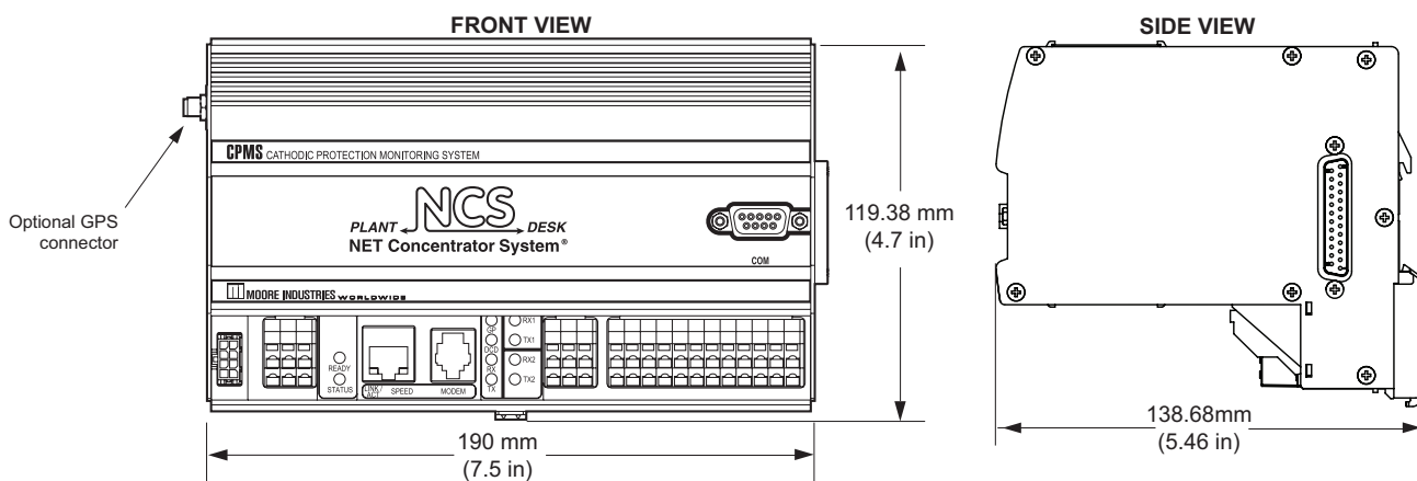
Figure 5. CPMS Dimensions (see the NCS NET Concentrator System data sheet for installation dimensions for expansion I/O).
