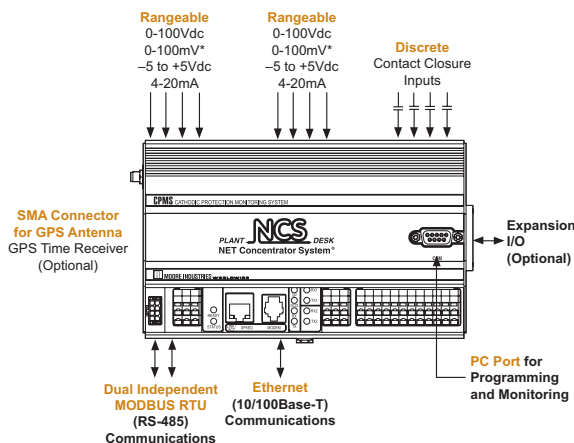
Figure 1. The stand-alone CPMS accepts four or eight analog inputs and four discrete (contact closure) inputs.
